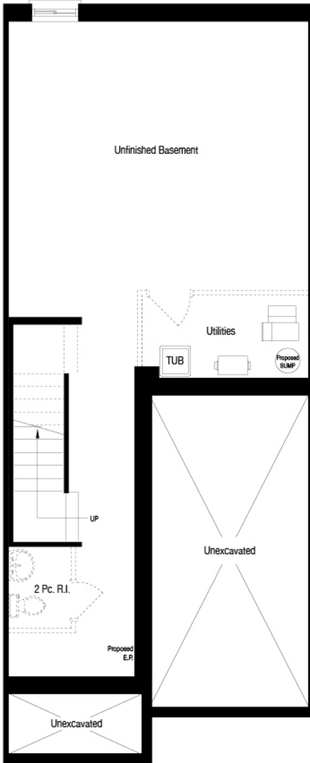
BASEMENT
