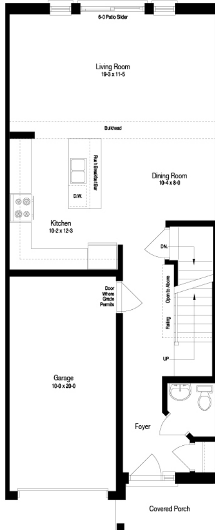
MAIN FLOOR
