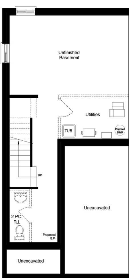
BASEMENT
