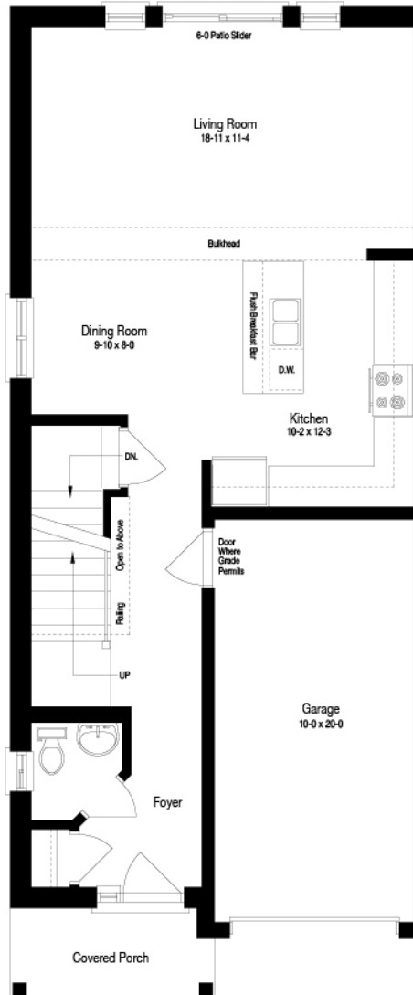
MAIN FLOOR
