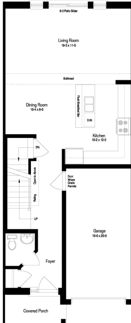
MAIN FLOOR
