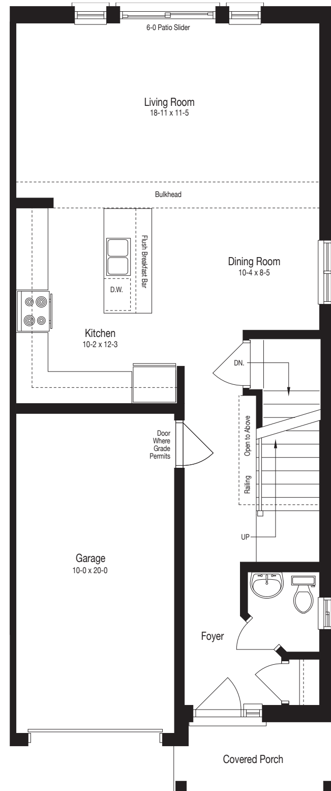
MAIN FLOOR
