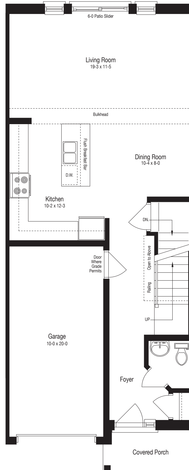
MAIN FLOOR
