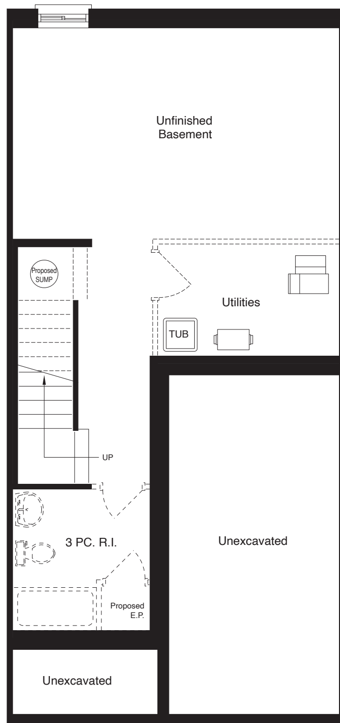
BASEMENT
