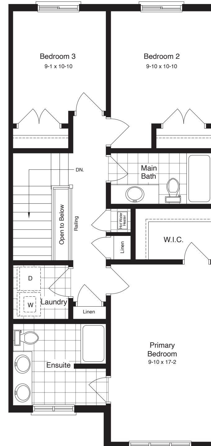
SECOND FLOOR
